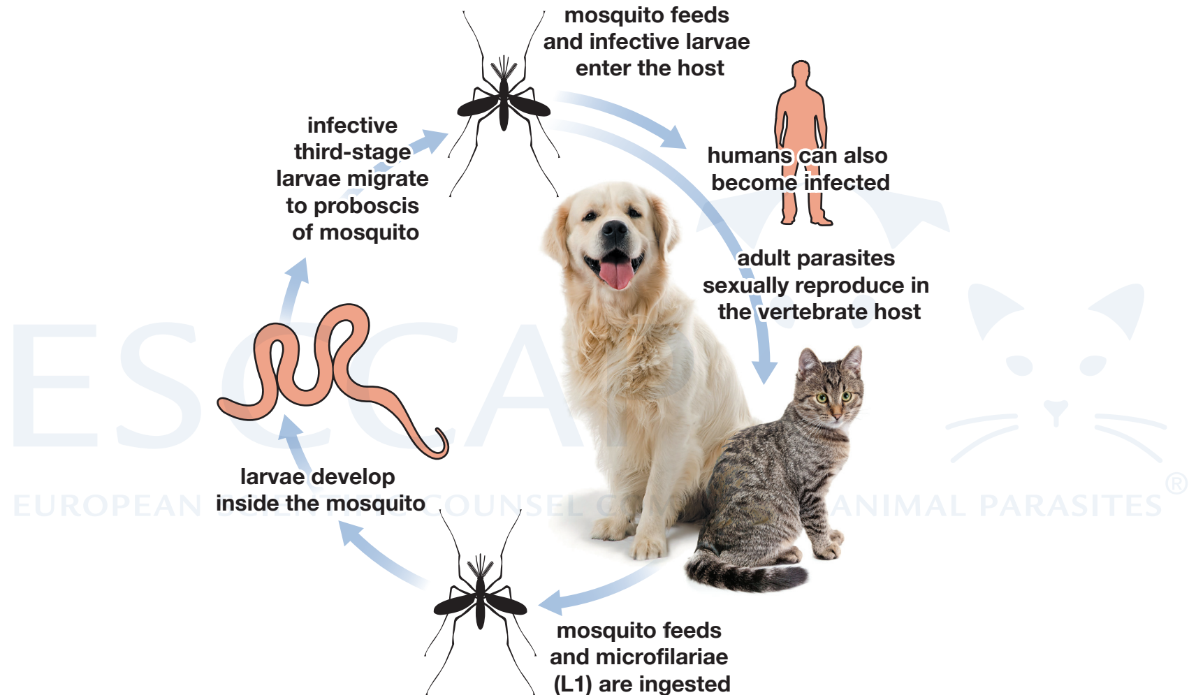
Heartworm ( Dirofilaria immitis ) life cycle
